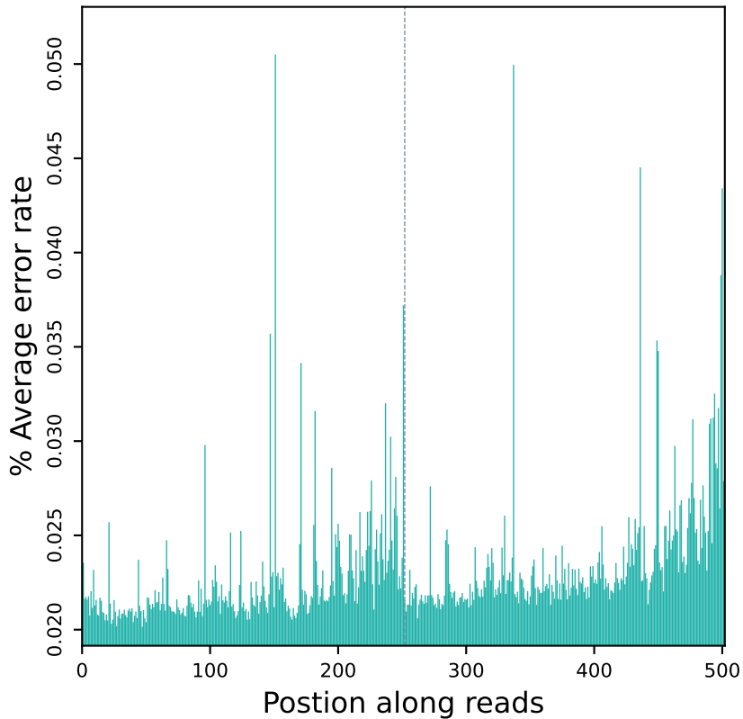
Error rate distribution along reads (R10320)
